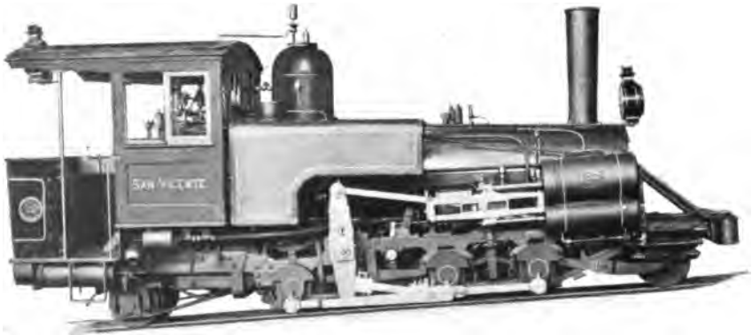
RACK AND ADHESION LOCOMOTIVE, CIA MINERA DE PEÑALES, MEXICO.
