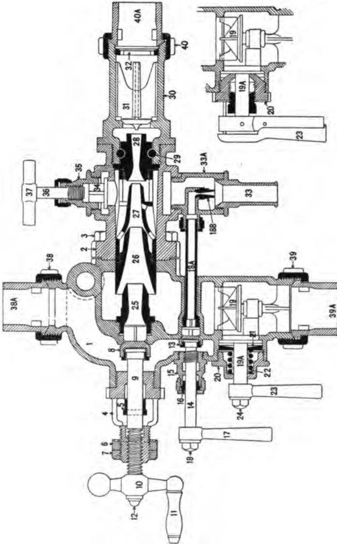
MONITOR INJECTOR.
