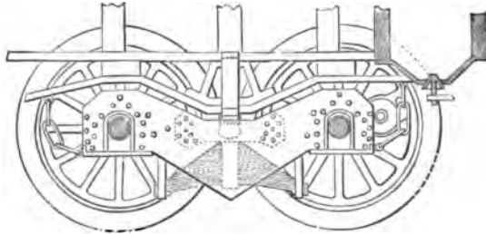
BALDWIN FLEXIBLE-BFAM TRUCK, 1842.—ELEVATION.
