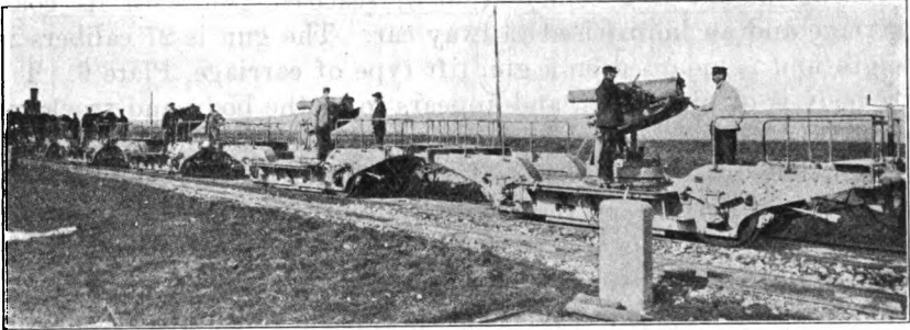
150-MM. HOWITZERS. PLATFORMS IN FIRING POSITION.
