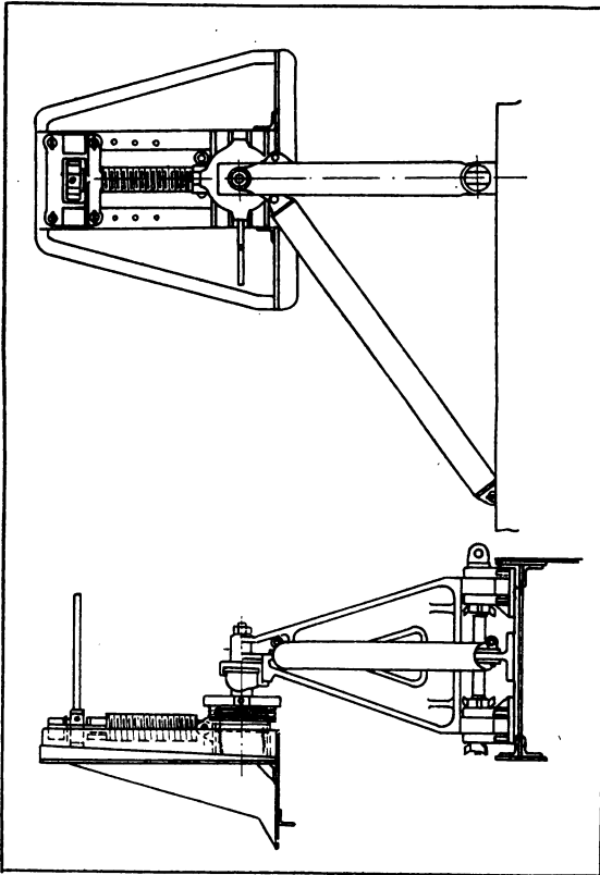
PLAN AND ELEVATION VIEWS OF OUTRIGGER FOR CAR MARK III.
