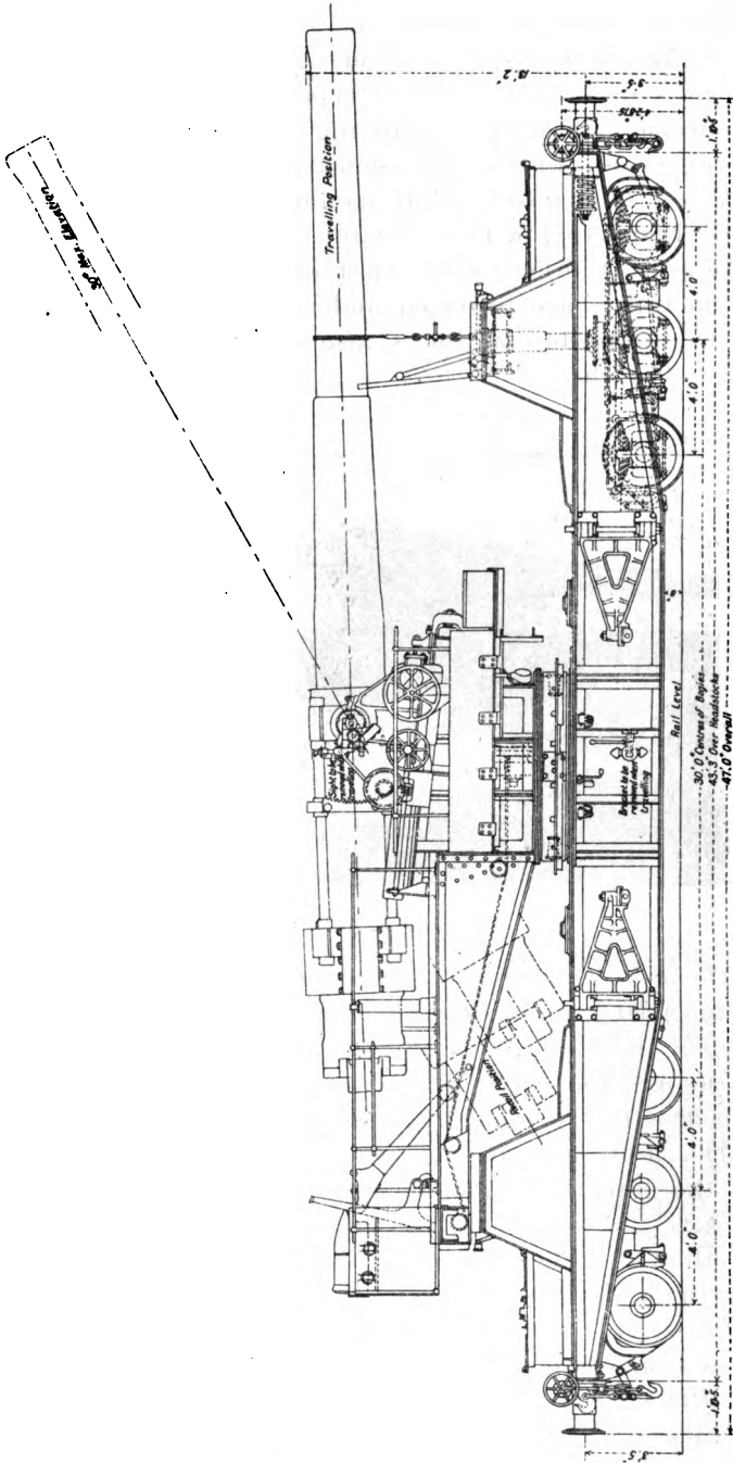
ASSEMBLY RIGHT SIDE ELEVATION BRITISH 9.2-INCH GUN MARK X ON A MARK III RAILWAY CAR, TRAVELING POSITION.
