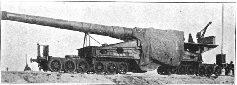
340-MM. GUN, MODEL 1912, ON ST. CHAMOND RAILWAY MOUNT, IN TRAVELING POSITION.
