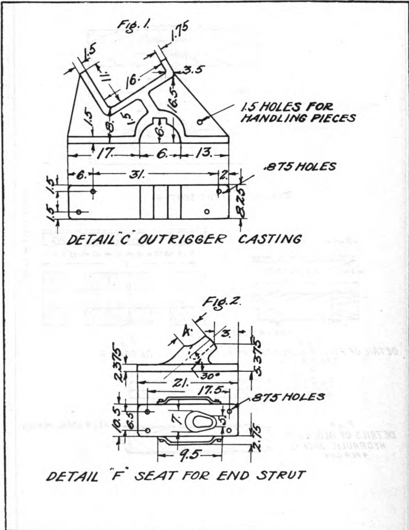
OUTRIGGER FLOAT DETAILS OF 240-MM. GUN, MODEL 1893-1896.
