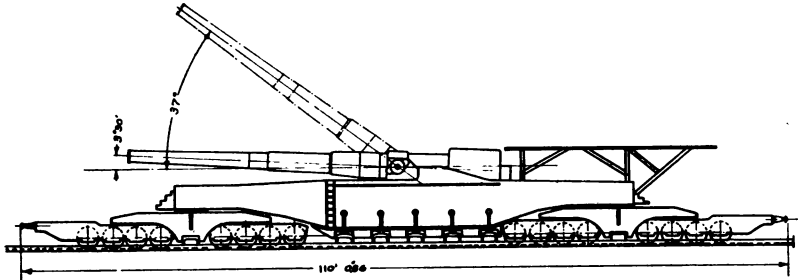
340-MM. GUN, MODEL 1912, ON SLIDING TYPE MOUNT.
