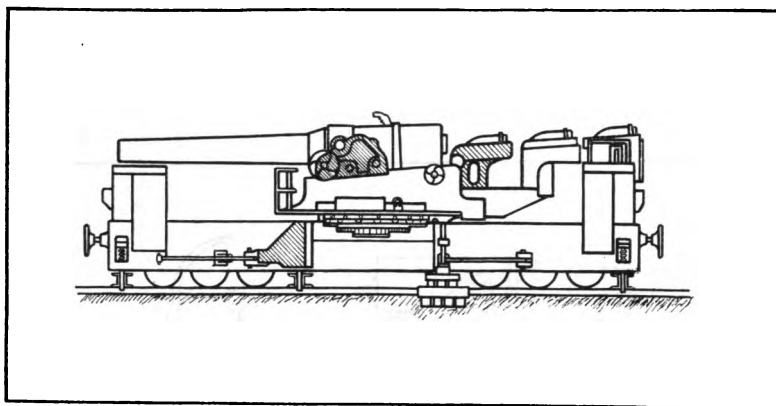
240-MM. GUN, MODEL 1870, 1884, 1887, ANCHORED FOR 360° TRAVERSE.
