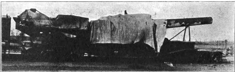
400-MM. HOWITZER MOUNT, TRAVELING POSITION.
