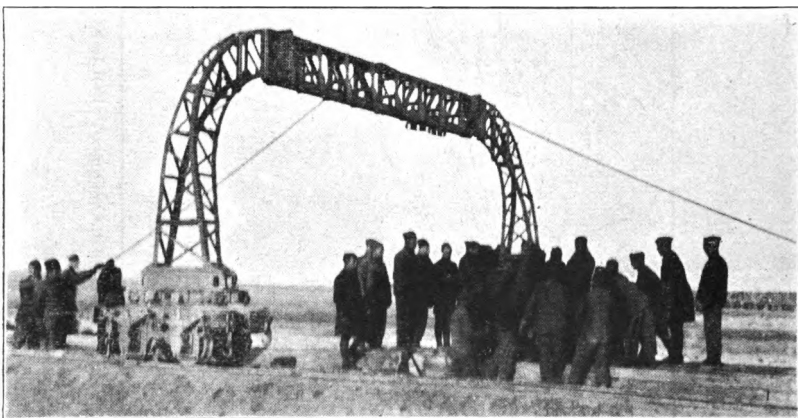
SETTING UP ROLLING BRIDGE.
