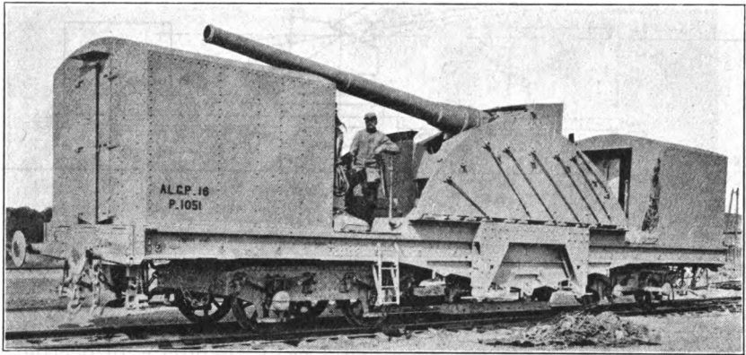
READY FOR TRANSPORTING.
